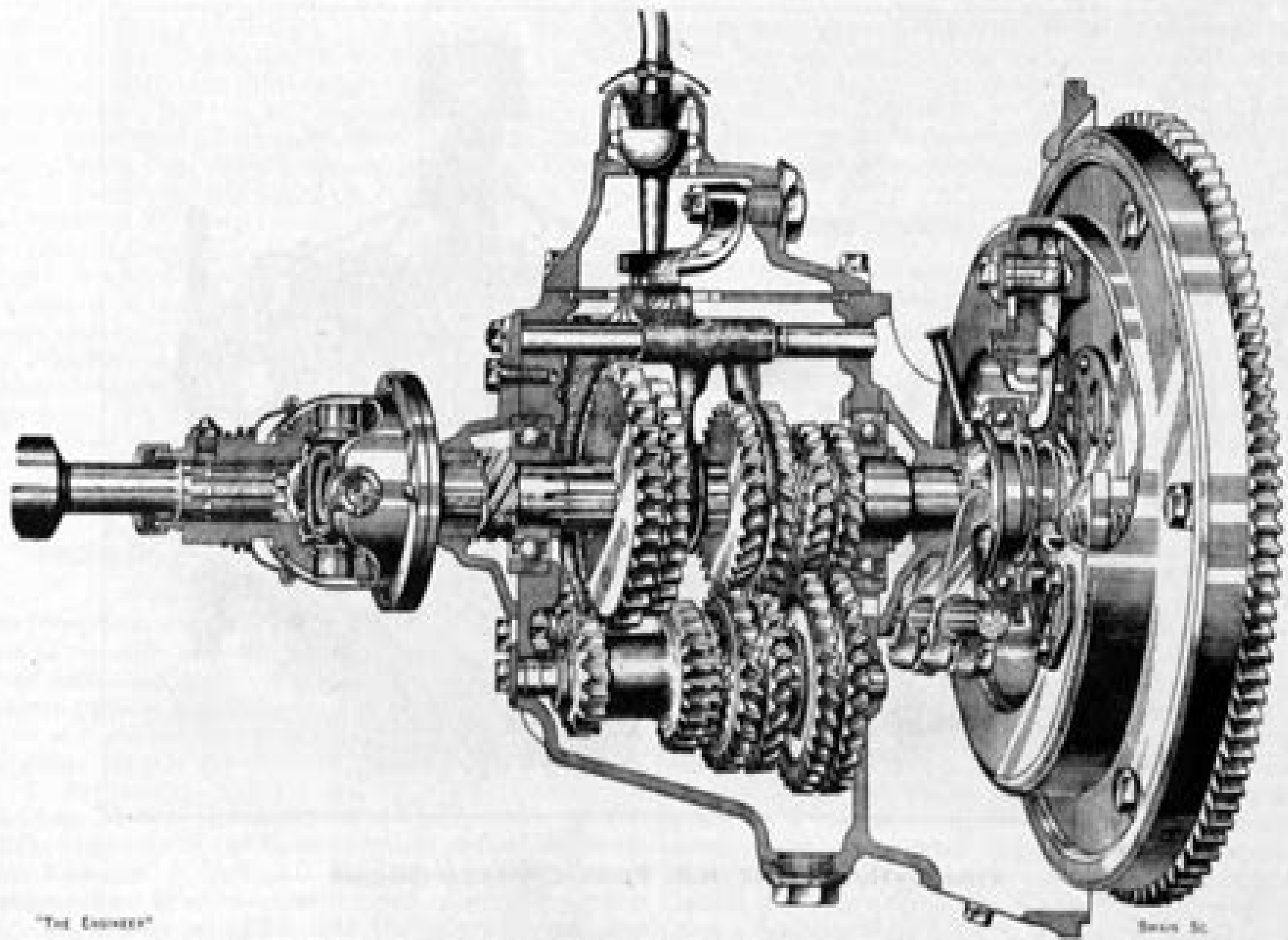
FIG. 16—GEAR-BOX DETAILS OF AUSTIN 10 H.P. CAR
